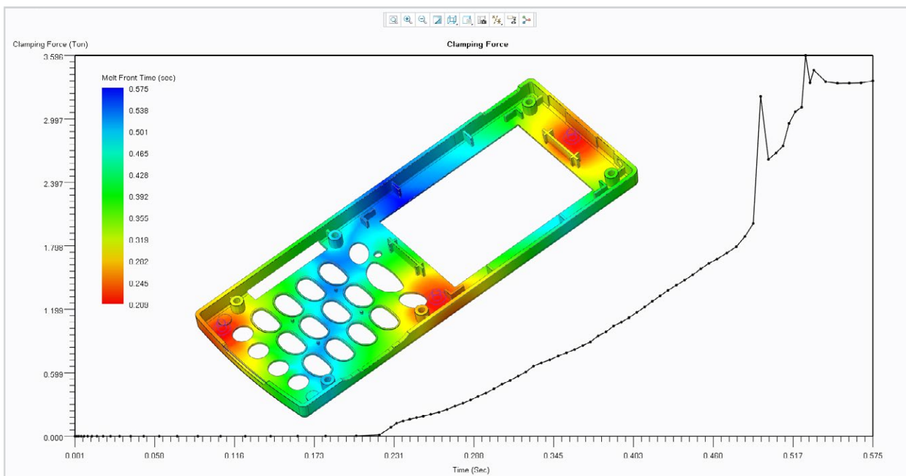
Simulate fill pressure with the PTC Creo Mold Analysis Extension
